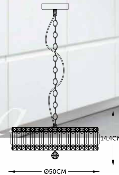
1024 Pendente Ravenna Cristal Clear 6*E14 40W Ø50*14.4cm
