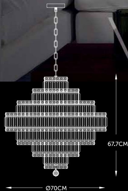
1025 Pendente Verona Cristal Clear 18*E14 40W Ø70*67.7cm
